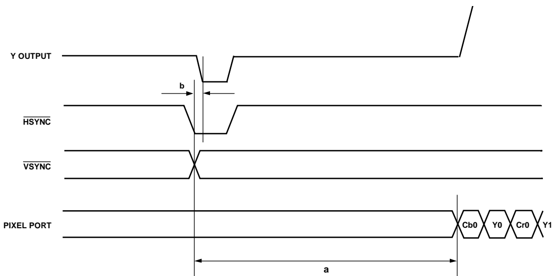
Figure 12. ED-SDR, 16-Bit 4:2:2 YCrCb ( \overline{\text{HSYNC}}/\overline{\text{VSYNC}} ) Input Timing Diagram
