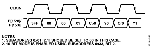
Figure 57. ED/HD-DDR Input Sequence (EAV/SAV)—Option A
