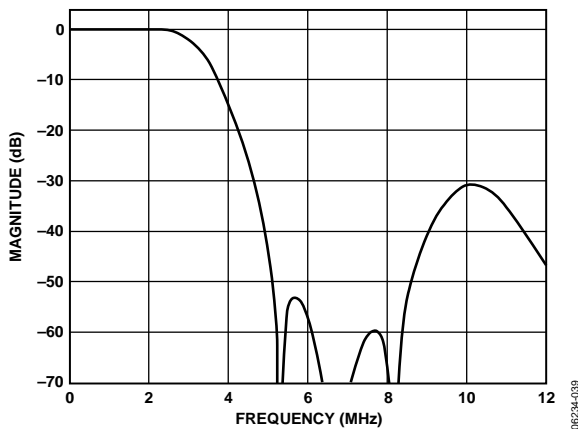
Figure 41. SD Chroma 2.0 MHz Low-Pass Filter Response
