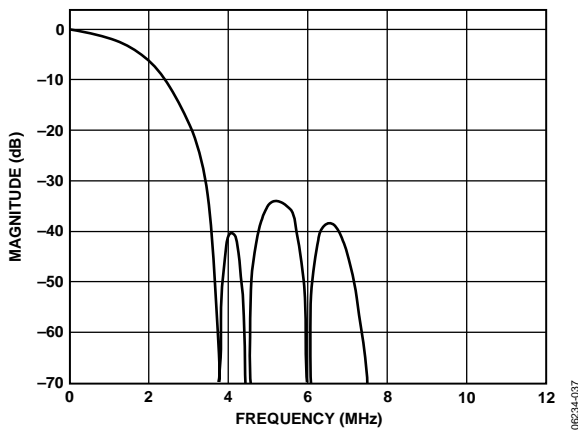
Figure 39. SD Luma QCIF Low-Pass Filter Response
