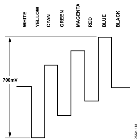
Figure 120. Pb Levels—NTSC
