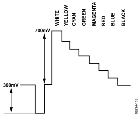
Figure 118. Y Levels—NTSC
