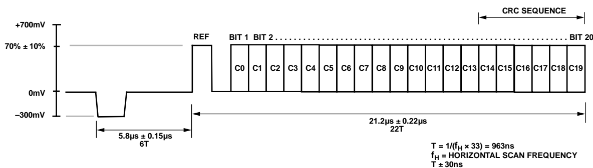
Figure 96. Enhanced Definition (525p) CGMS Waveform
