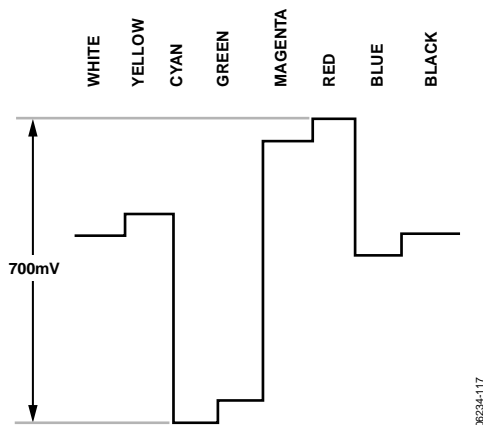
Figure 119. Pr Levels—NTSC
