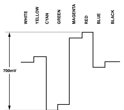
Figure 122. Pr Levels—PAL
