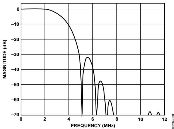
Figure 40. SD Chroma 3.0 MHz Low-Pass Filter Response
