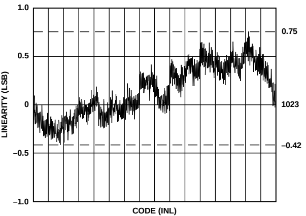
Figure 18. Typical Linearity
