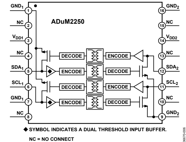
Figure 6. ADuM2250 Block Diagram
