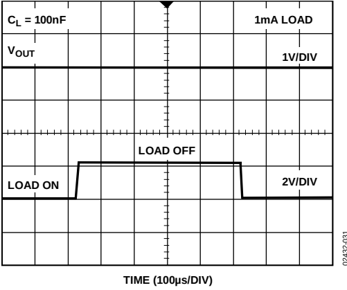
Figure 30. ADR421 Load Transient Response, C_L = 100nF
