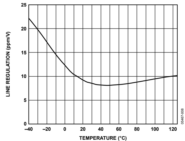
Figure 13. ADR360 Line Regulation vs. Temperature, V_{IN} = 2.45 \text{ V to } 15 \text{ V}
