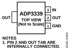
Figure 3. 3-Lead SOT-223 Pin Configuration
