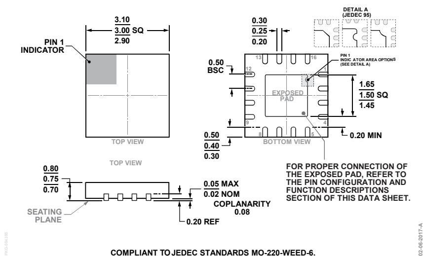
COMPLIANT TO JEDEC STANDARDS MO-220-WEED-6. Figure 36. 16-Lead Lead Frame Chip Scale Package [LFCSP] 3 mm × 3 mm Body and 0.75 mm Package Height (CP-16-27) Dimensions shown in millimeters
