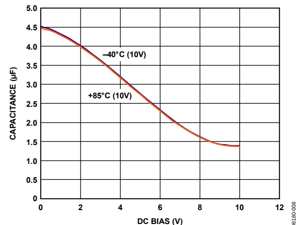
Figure 33. DC Bias Characteristic of a 10 V, 4.7 \mu\text{F} Ceramic Capacitor
