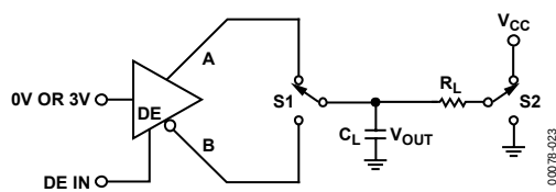
Figure 23. Driver Enable/Disable
