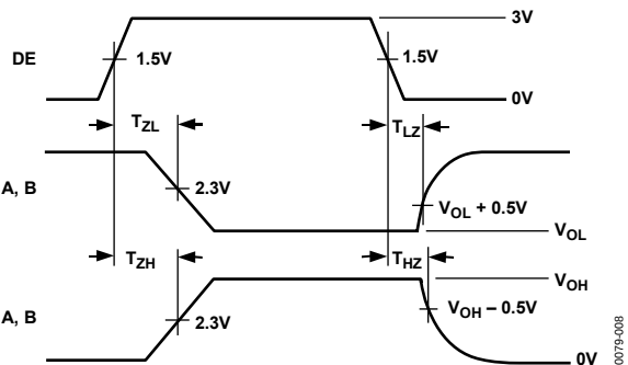
Figure 13. Driver Enable/Disable Timing
