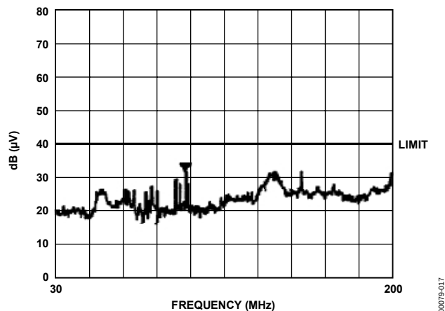
Figure 22. Radiated Emissions
