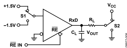
Figure 34. Receiver Enable/Disable
