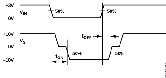
Figure 17. Switching Times
