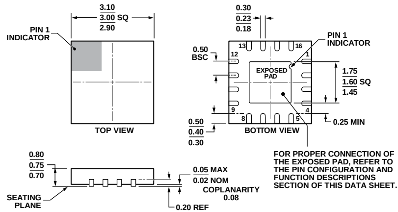
Figure 37. 16-Lead Lead Frame Chip Scale Package [LFCSP_WQ] 3 mm x 3 mm Body, Very Very Thin Quad (CP-16-22) Dimensions shown in millimeters
