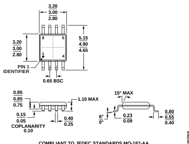
Figure 33. 8-Lead Mini Small Outline Package [MSOP] (RM-8) Dimensions shown in millimeters
