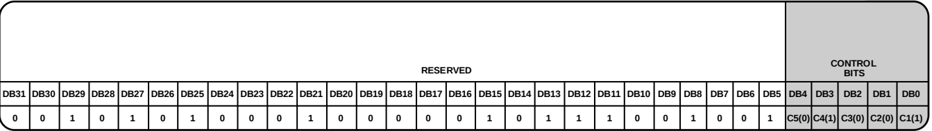
Figure 28. Register 9 (R9)
