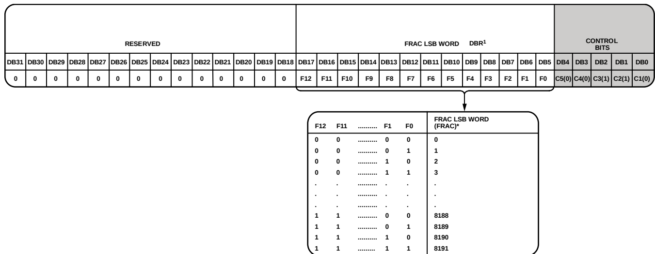
Figure 25. Register 6 (R6)
