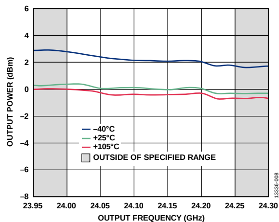
Figure 8. LO Output Power vs. Output Frequency
