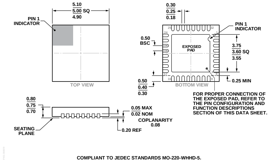
Figure 32. 32-Lead Lead Frame Chip Scale Package [LFCSP] 5 mm × 5 mm Body and 0.75 mm Package Height (CP-32-12)
