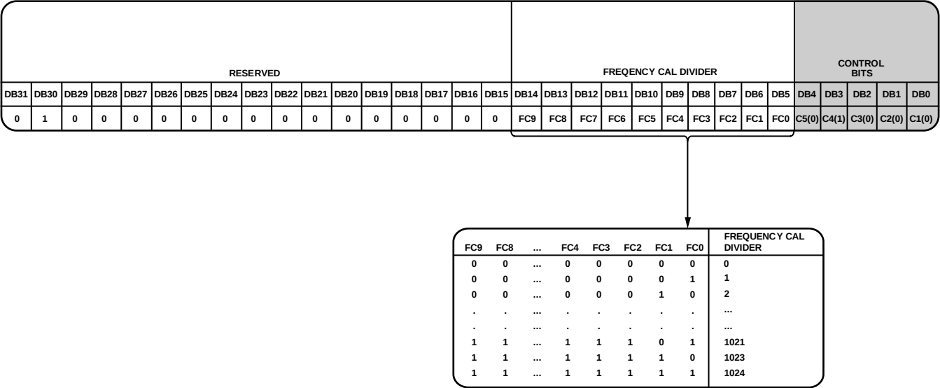
Figure 27. Register 8 (R8)
