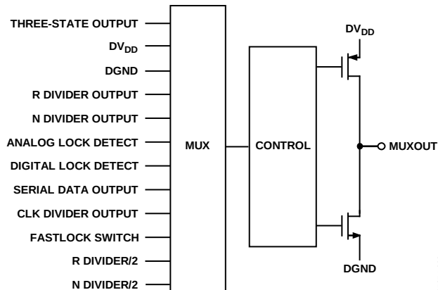
Figure 15. MUXOUT Schematic
