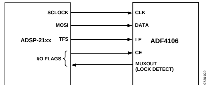
Figure 24. ADSP-21xx-to-ADF4106 Interface
