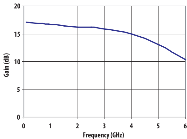
Figure 5. Gain vs Frequency at I_d = 60\text{ mA} .
