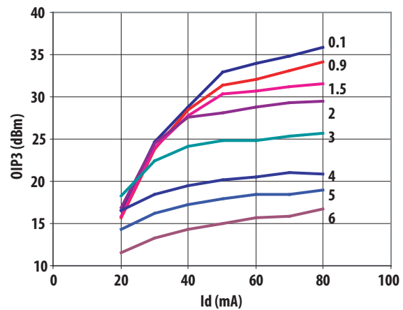
Figure 16. OIP3 vs Id and Frequency (GHz).
