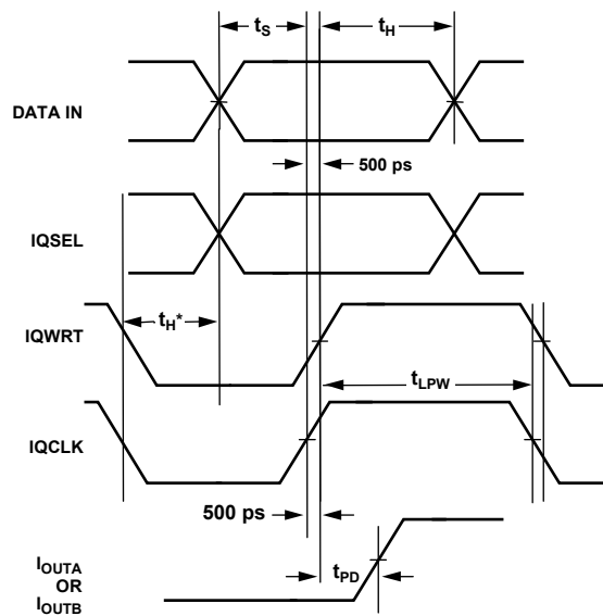
Figure 64. 5 V or 3.3 V Interleaved Mode Timing
