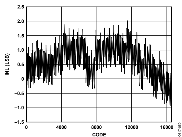
Figure 50. Typical INL
