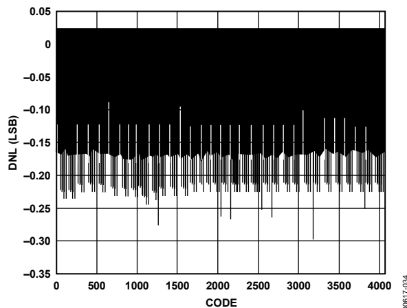
Figure 34. Typical DNL
