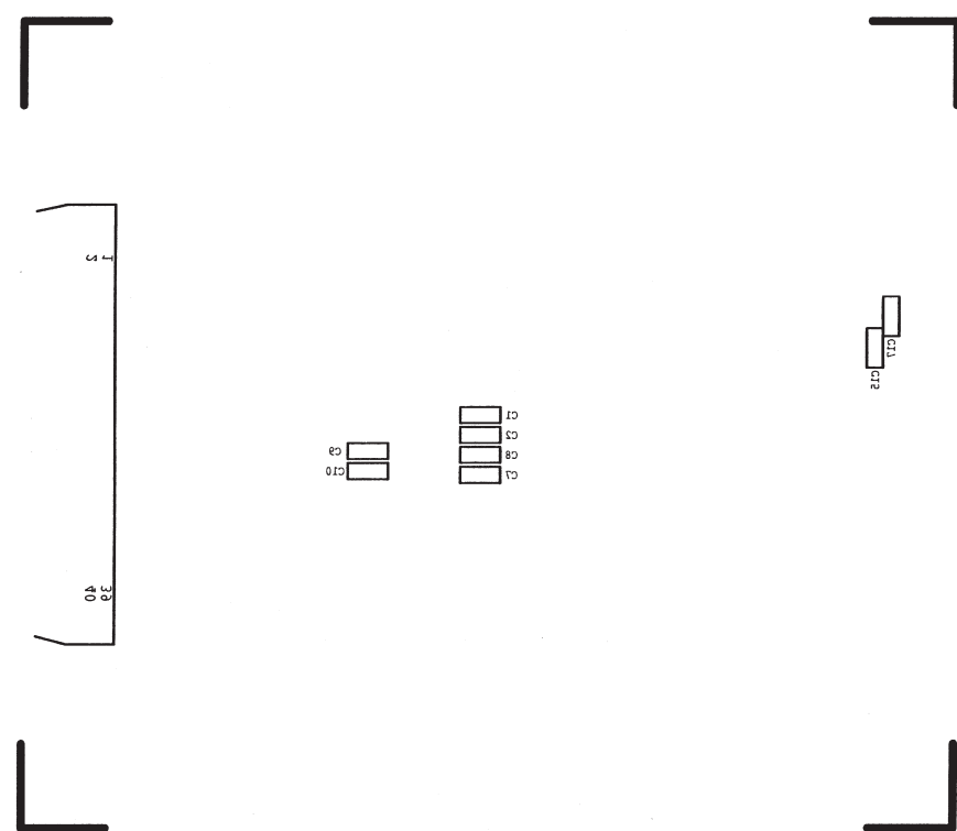
Figure 30. Silkscreen Layer—Bottom
