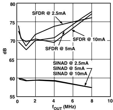
TPC 7. SINAD/SFDR vs. I_{\text{OUTFS}} (DC to f_{\text{DATA}}/2 , Differential Output)
