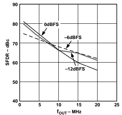
Figure 5. SFDR vs. f_{OUT} @ 50 MSPS
