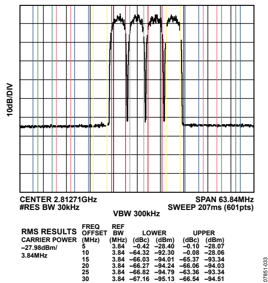
Figure 33. Typical Four-Carrier WCDMA ACLR Performance at 2.8 GHz, f_{DAC} = 2457.6 \text{ MSPS} (Third Nyquist Zone)
