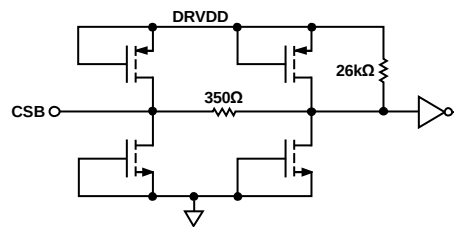
Figure 61. Equivalent CSB Input Circuit
