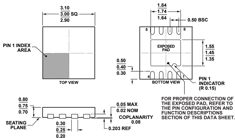
Figure 44. 8-Lead Lead Frame Chip Scale Package [LFCSP_VD]
