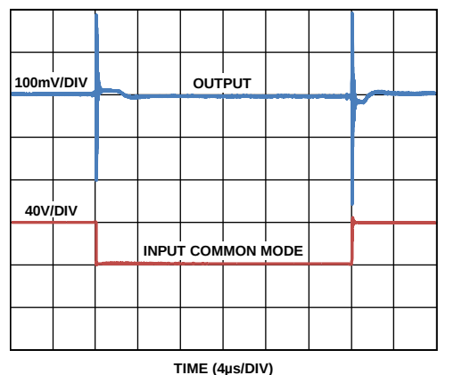
Figure 18. Input Common-Mode Step Response ( V_S = 5V , Inputs Shorted)
