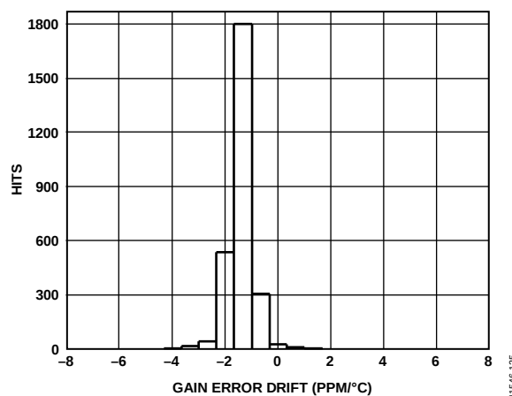
Figure 25. Gain Drift Distribution
