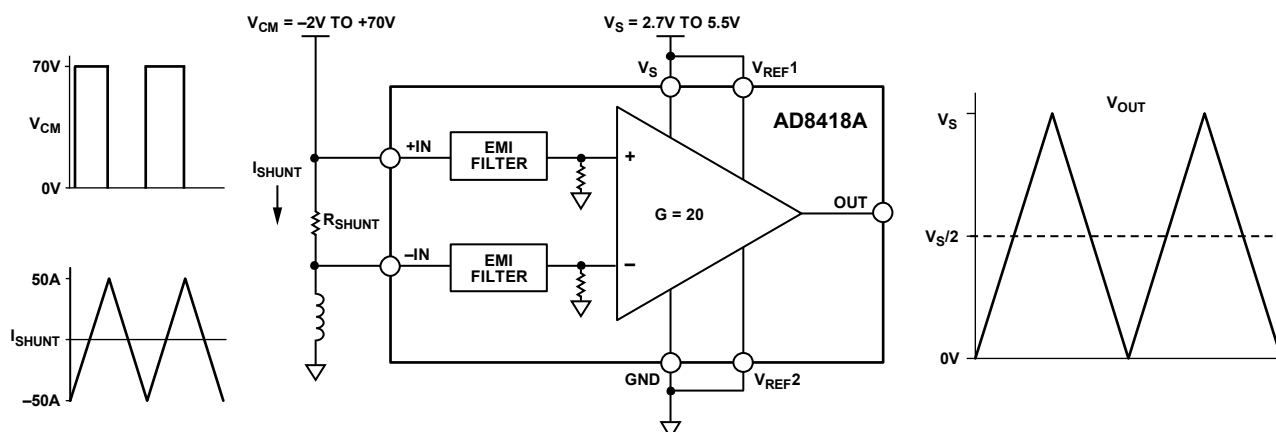
Figure 29. Typical Application
