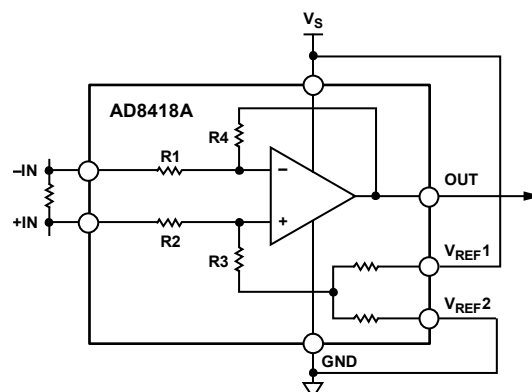
Figure 33. Split Supply
