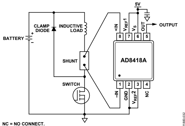
Figure 37. Low-Side Switch
