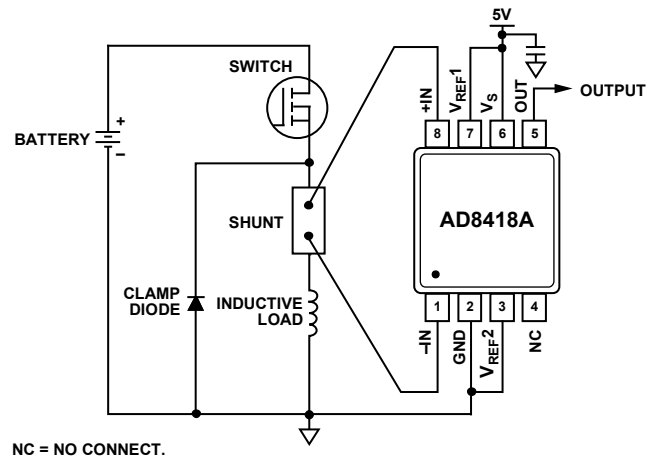
Figure 38. High-Side Switch
