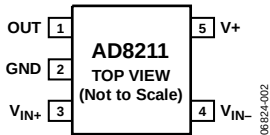
Figure 3. Pin Configuration
