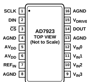
Figure 3. Pin Configuration
