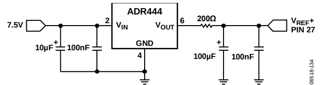
Figure 54. Reference Connection
