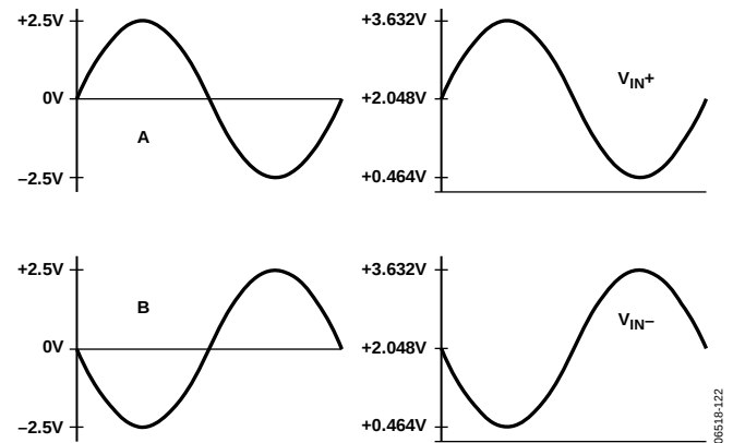
Figure 38. Differential Amplifier Signal Conditioning
