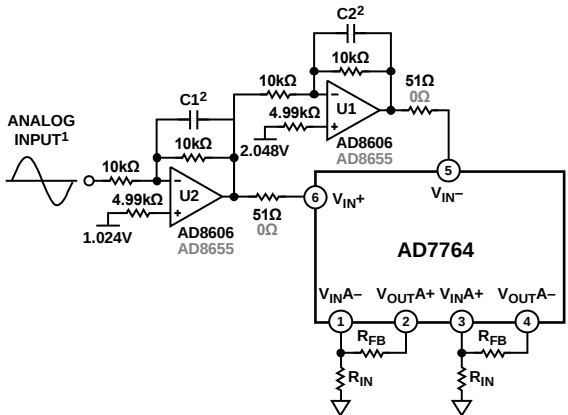
Figure 42. Driving the AD7764 Modulator Inputs Directly from a Single-Ended Source (On-Board Differential Amplifier Powered Down)
