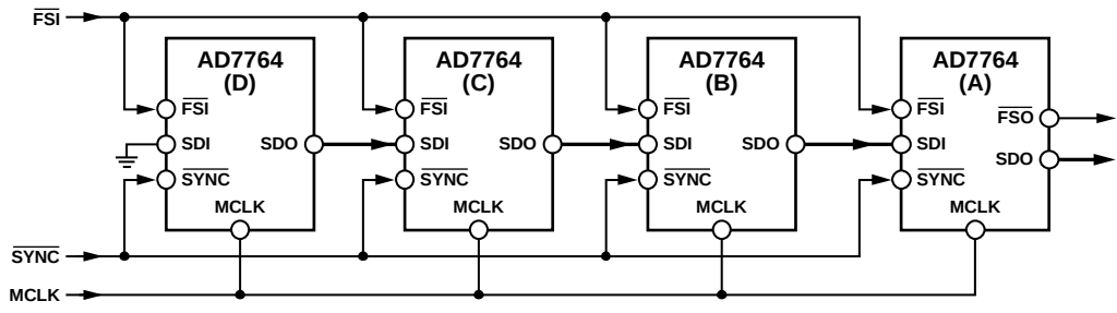
Figure 47. Daisy-Chaining Four Devices in Decimate 128× Mode Using a 40 MHz MCLK Signal
