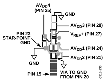
Figure 53. Supply Decoupling
