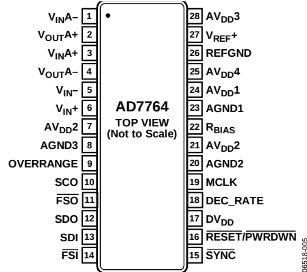
Figure 5. Pin Configuration
