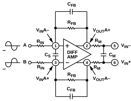
Figure 37. Differential Amplifier Configuration
