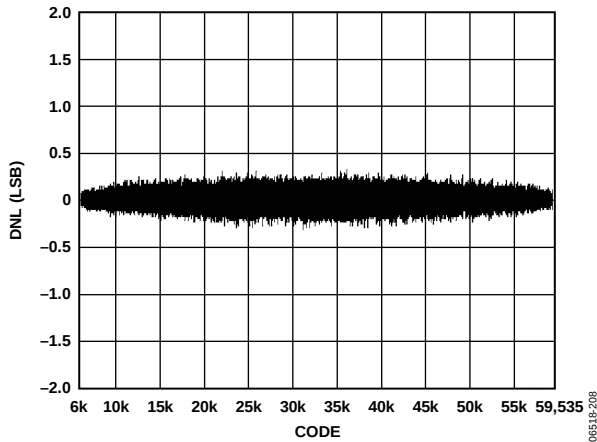
Figure 24. DNL Plot
