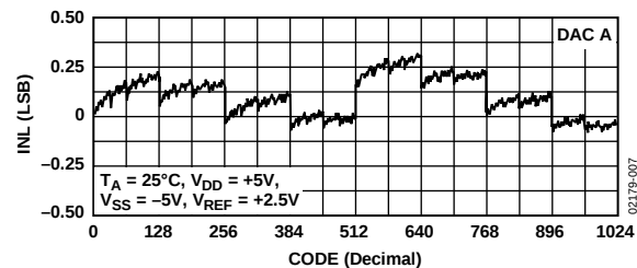
Figure 7. AD7399 INL vs. Code ( T_A = 25^\circ C )
