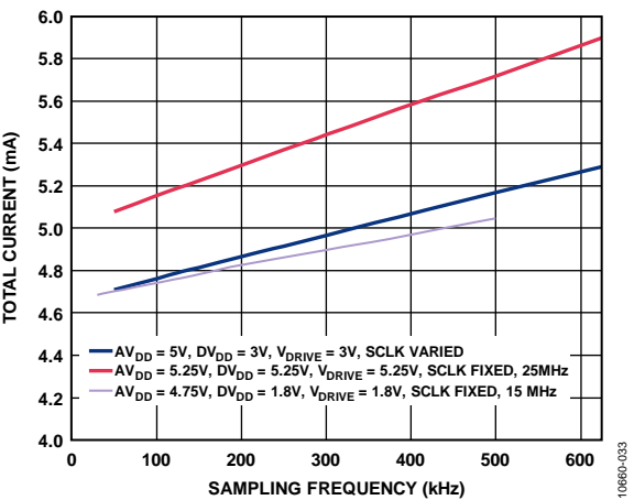
Figure 30. Total Supply Current vs. Throughput Rate
