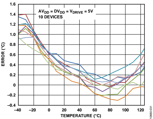
Figure 28. Temperature Sensor Error vs. Temperature
