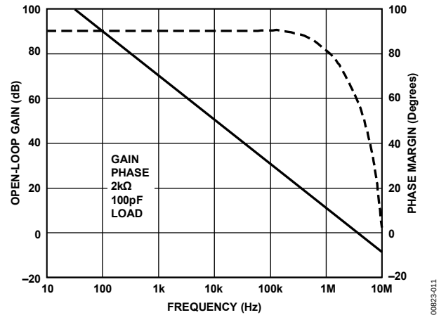
Figure 11. Open-Loop Gain and Phase Margin vs. Frequency
