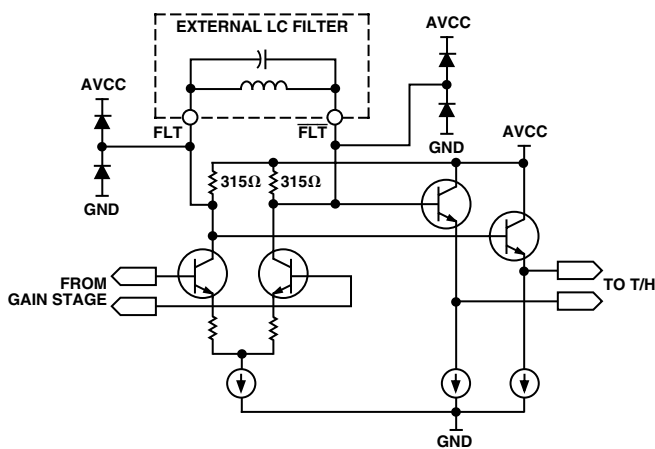
Figure 5. Resonant (LC Noise Filter) Port
