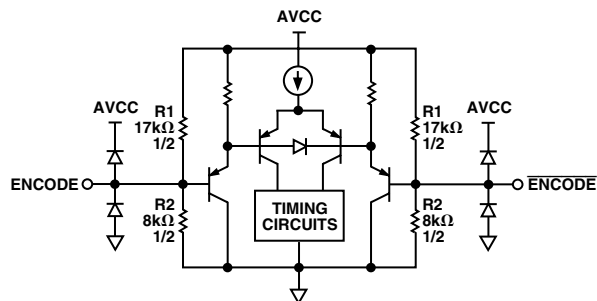
Figure 6. Encode Inputs
