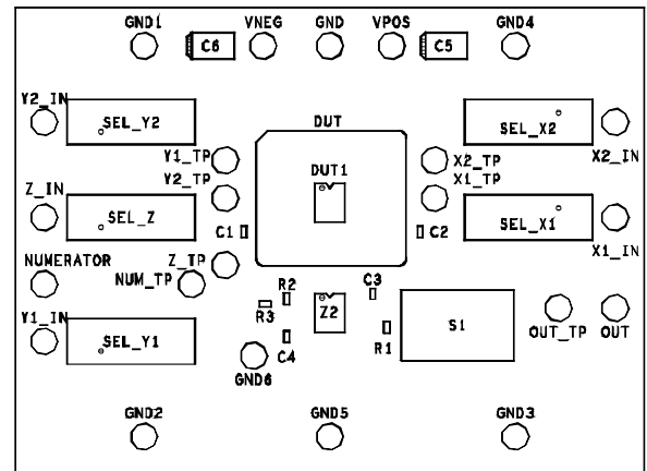
Figure 48. AD633-EVALZ Assembly
