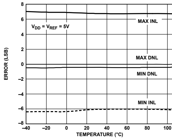
Figure 24. INL Error and DNL Error vs. Temperature
