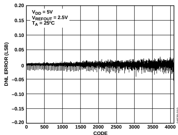
Figure 11. DNL—AD5620-2/AD6520-3
