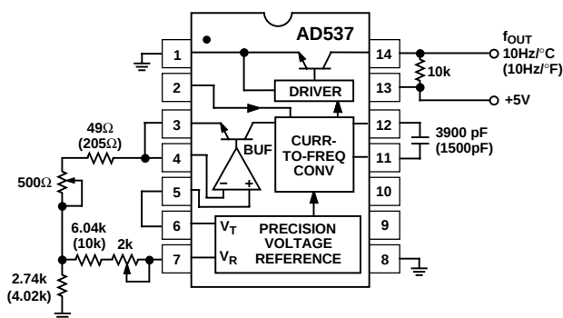
Figure 9. Offset Temperature Scale Converters Centigrade and (Fahrenheit) to Frequency
