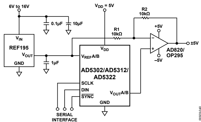
Figure 40. Bipolar Operation Using the AD5302/AD5312/AD5322
