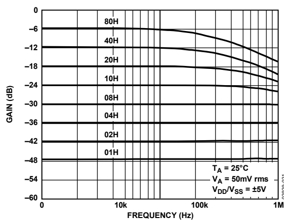
Figure 23. Gain vs. Frequency vs. Code, R_{AB} = 200\text{ k}\Omega
