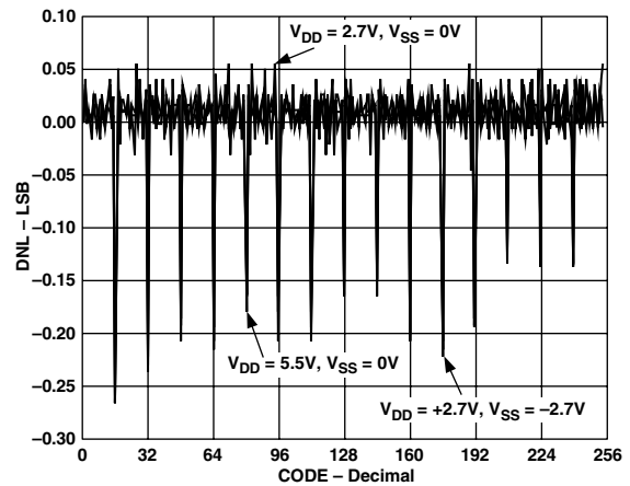
TPC 5. AD5200 10 kΩ DNL vs. Code
