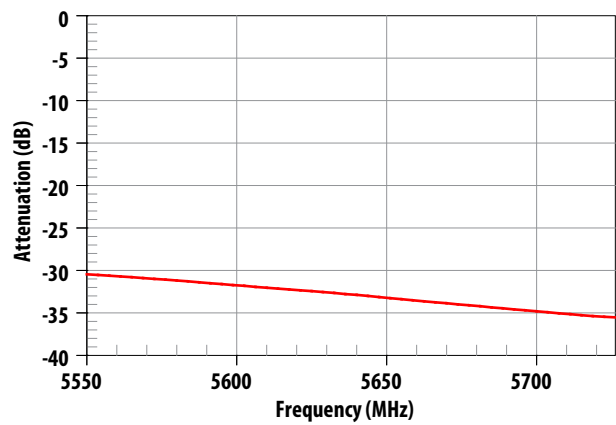
Figure 12. PCS Ant-Tx Rejection at Tx Third Harmonic (Dual Antenna, Note1).
