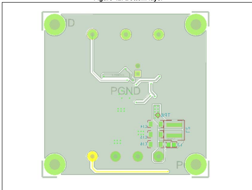
Figure 42. Bottom layer
