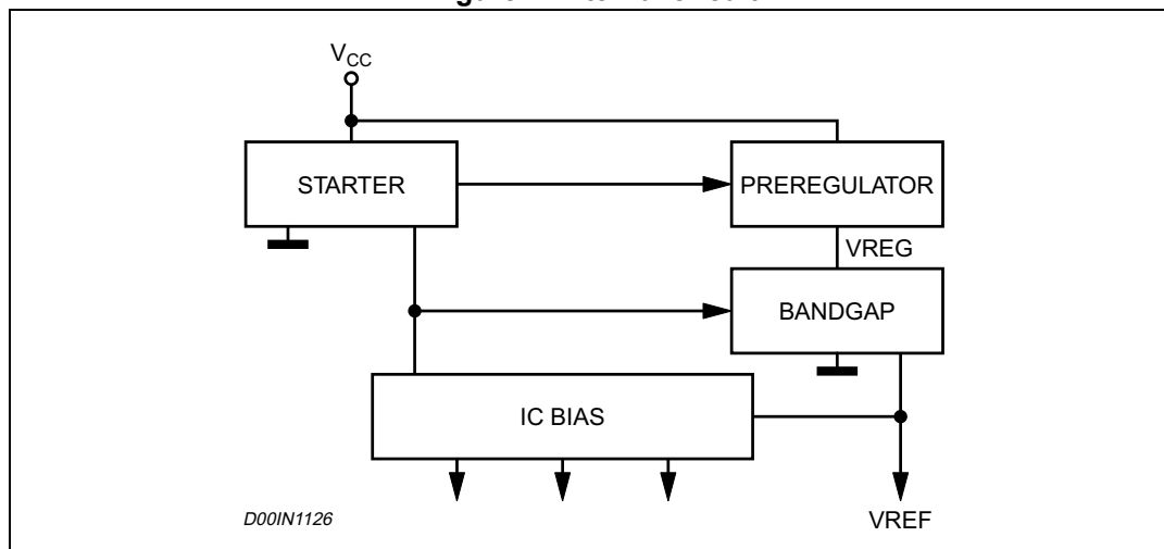
Figure 4. Internal circuit
