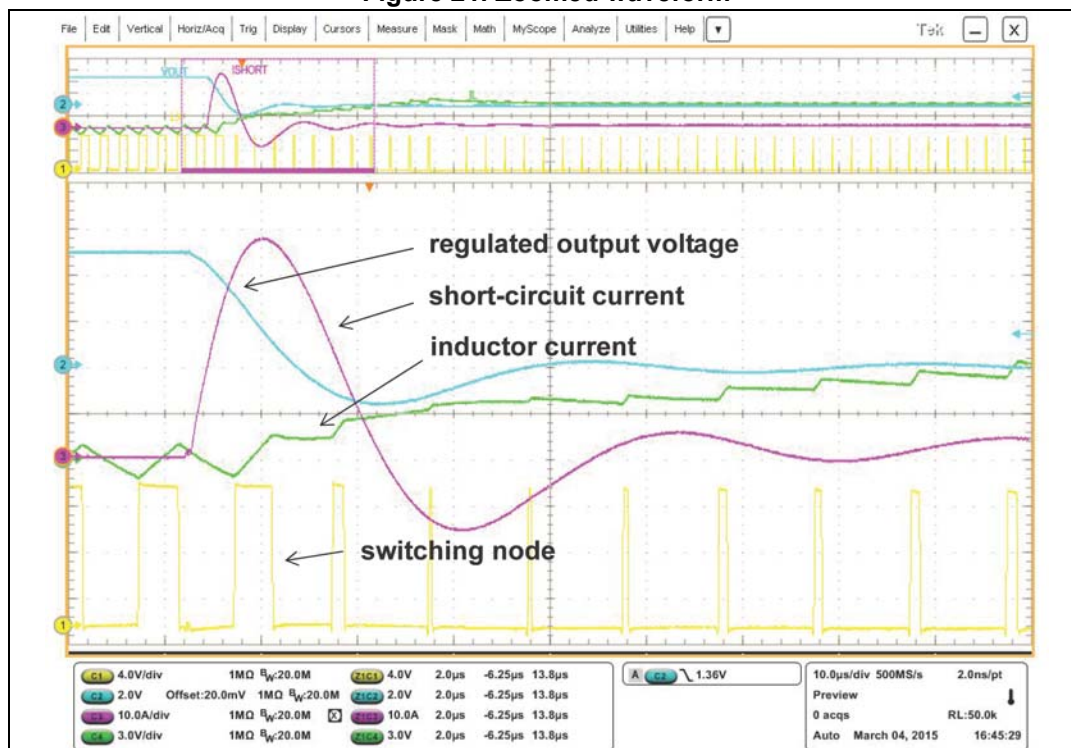
Figure 21. Zoomed waveform
