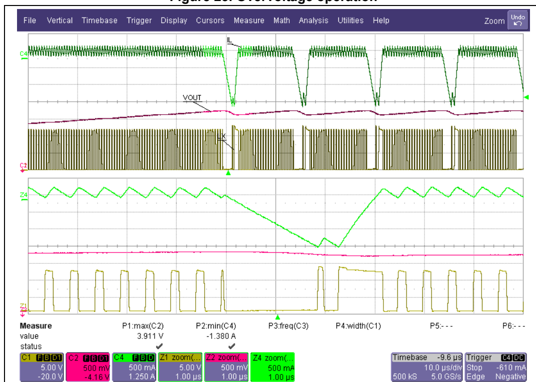
Figure 23. Overvoltage operation
