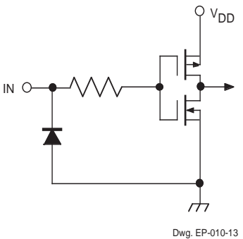
CLOCK and SERIAL DATA IN
