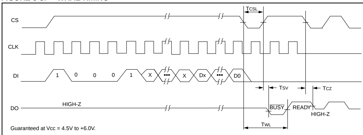
FIGURE 3-8: WRAL TIMING
