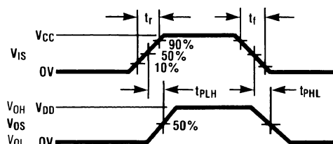
Figure 4. t_{\text{PHL}} , t_{\text{PLH}} Propagation Delay Time Signal Input to Signal Output
