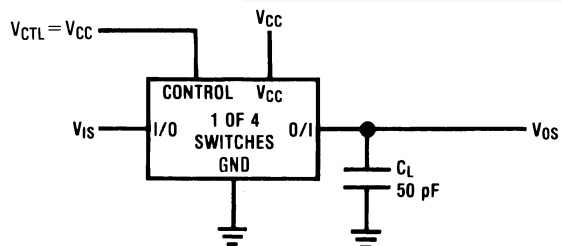
Figure 4. t_{\text{PHL}} , t_{\text{PLH}} Propagation Delay Time Signal Input to Signal Output
