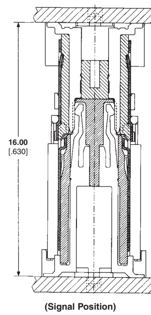
16mm Height
