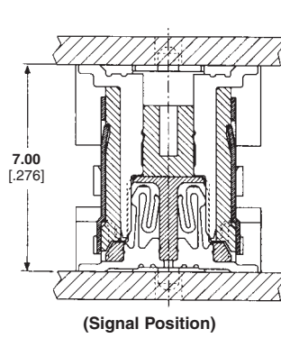
7mm Height
