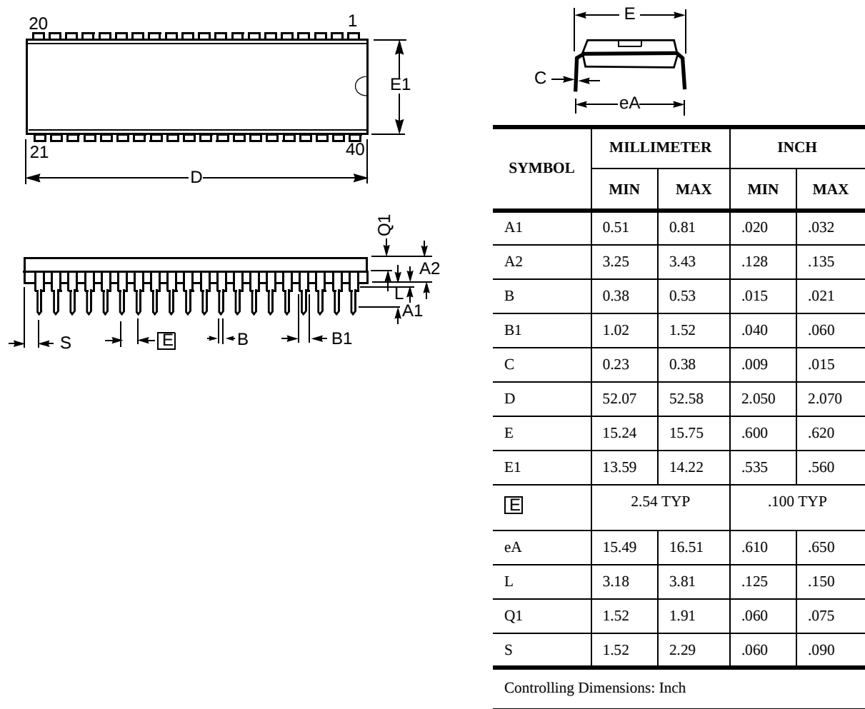
Figure 37 displays the 40-pin Dual-Inline Package (DIP).
