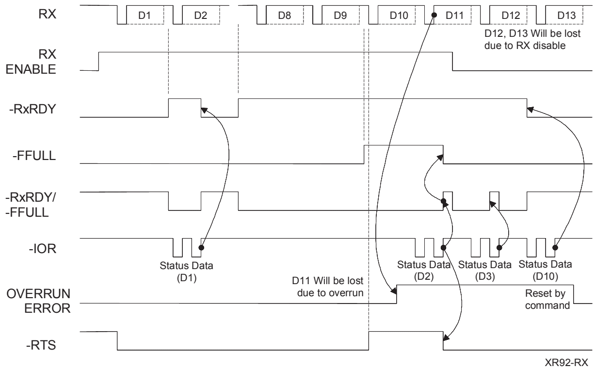
Figure 6: Receive Timing
