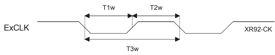
Figure 9: External clock Timing
