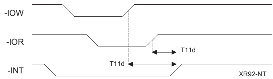
Figure 8: Interrupt Timing
