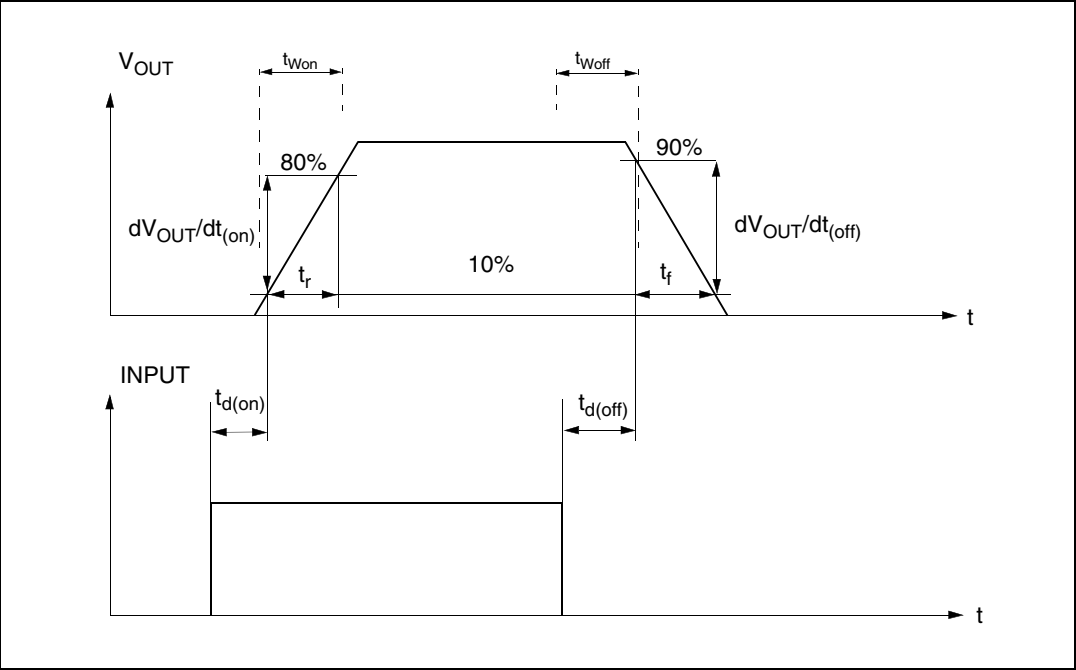
Figure 6. Switching characteristics
