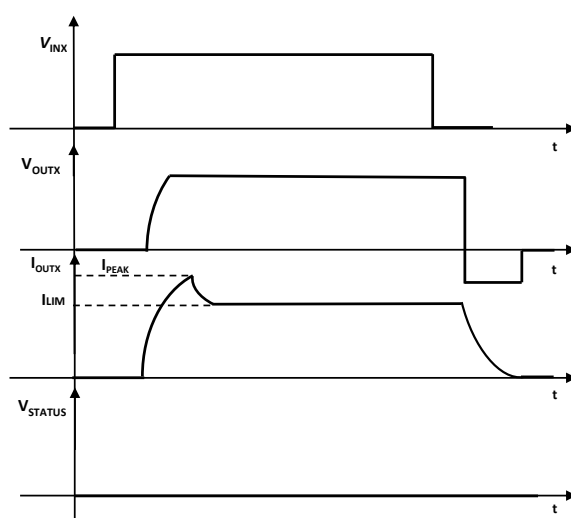
Figure 11. Switching on heavy inductive Load
