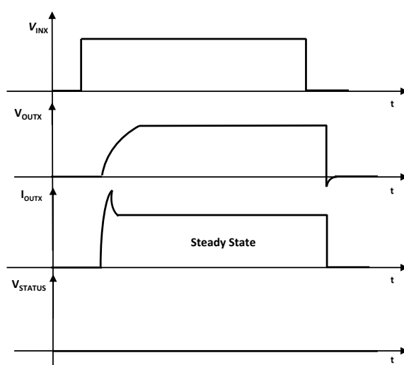
Figure 9. Switching on Bulb Lamp Load
