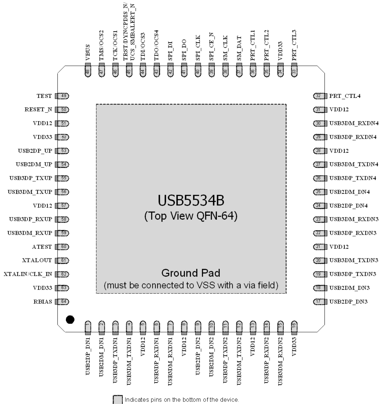
Figure 3.1 USB5534B 64-Pin QFN
