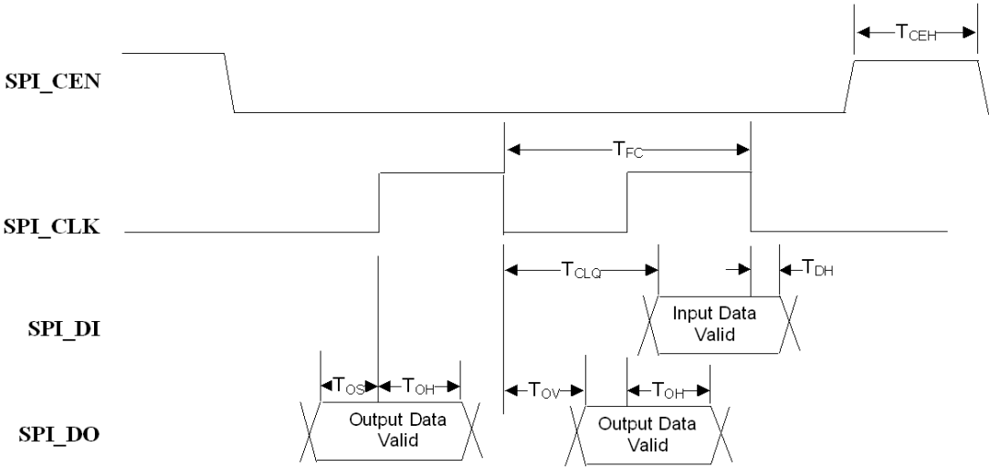
Figure 7.3 SPI Timing
